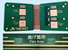
FR4-Flex基板断面 X-section of Semi-flex PWB
