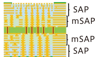
CoWoP Technology ※Chip on Wafer on PCB
