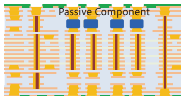
Embedded PCB Technology
