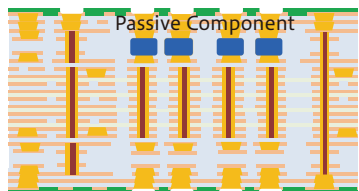
Embedded PCB Technology
