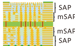
CoWoP Technology ※Chip on Wafer on PCB
